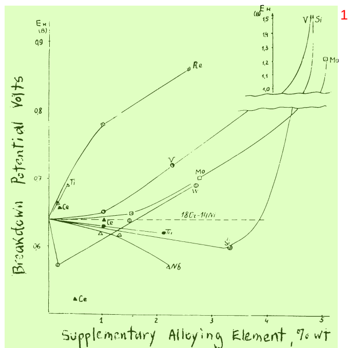
Figure 3—Effect of alloying elements on the breakdown potential ( E_b ) of 18Cr-14Ni steel in 0.1N NaCl. Temperature, 25 C
